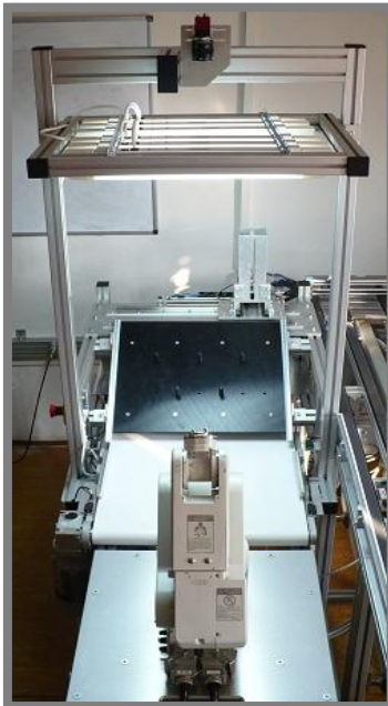
Guidance of Mitsubishi Melfa manipulator
